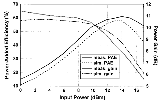
Fig. 14. Measured and simulated PAE and power gain versus input power for the combined approach power amplifier.
