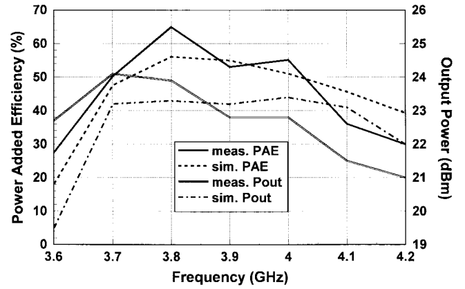
Fig. 13. Measured and simulated PAE and output power versus frequency for the broad-band power amplifier integrated with slot and periodic structure.
