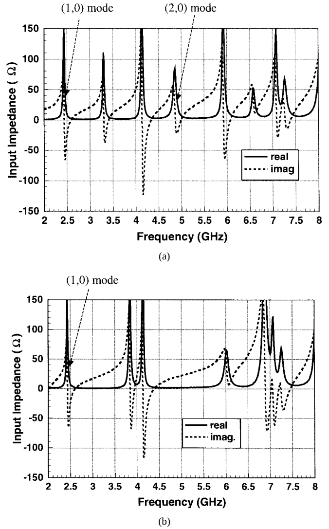
Fig. 4. (a) Measured input impedance of patch antenna. (b) Patch antenna with shorting pins. In both cases, the antenna is 1550-mil long and 2320-mil wide.
